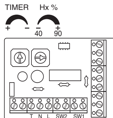
Detail hygrosatu
